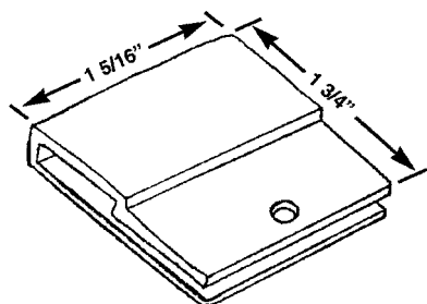
AWV 65 SUPERIOR PB GUIDE
