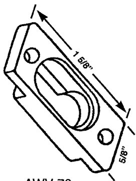
AWV 70 BALANCE BLOCK
