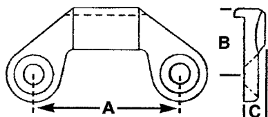
WLK 18 A B C 1 3/8" 39/64" 5/32"
