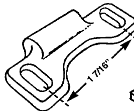
WLK 68 KEEPER
