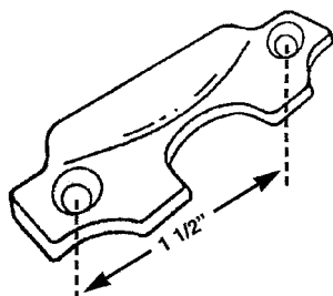
WLK 66 WEDGE BLOCK
