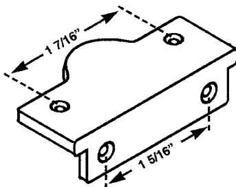
WLK 94
