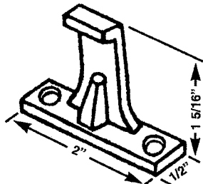
WPA 141 HOLDER
