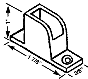
WPA 140 KEEPER
