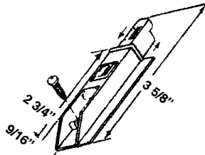
CDF 97 GLIDEALL BOTTOM GUIDE
