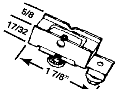
CDF 37 TOP PIVOT BRACKET
