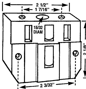
CDF 110 CORNER CONNECTOR FOR MIRROR DOOR
