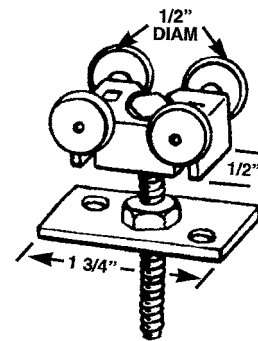
CDF 138 COX 4-WHEEL CARRIER
