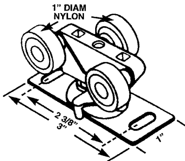
CDF 131 TRICYCLE HANGER
