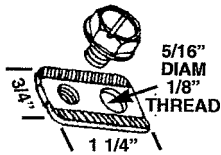
CDF 703 LEIGH/MONARCH PIVOT BKT
