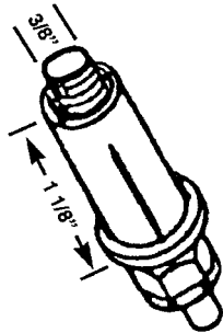
CDF 128 COX ROLLER GUIDE
