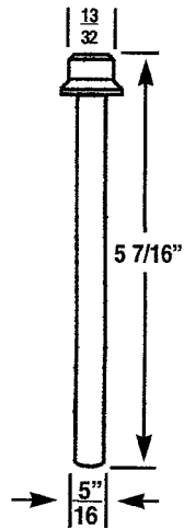
CDF 682 LEIGH MONARCH PIN W/CAP
