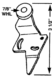
CDB 4 OVAL HANGER
