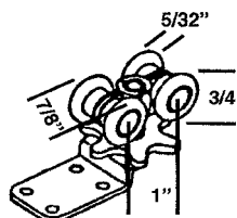
CDB 25 ADJ. TOP MOUNT HANGER
