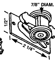
CDB 106 POCKET 2-WHEEL
