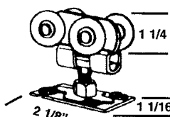
CDB 26 HEAVY DUTY HANGER
