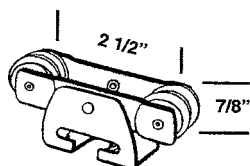
CDB 30 CARRIER
