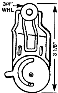
CDB 168 7/16" OFFSET
