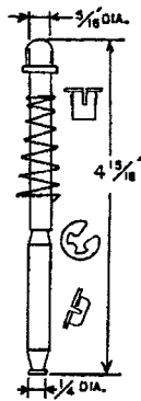
CDF 637 FLOATAWAY OLD TOP GUIDE
