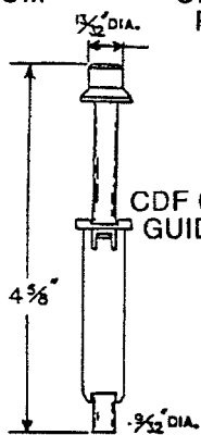
CDF 636 FLOATAWAY OLD TOP PIVOT
