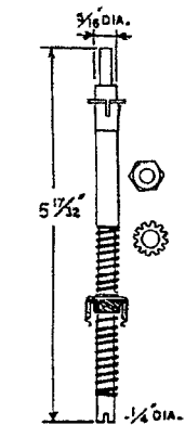
CDF 635 FLOATAWAY OLD BOTTOM PIVOT
