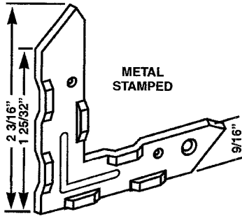
SSP 22 CORNER KEY
