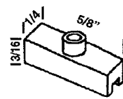
SWP 30 ALENCO SLIDE GUIDE
