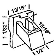
HWP 494 LONG BRACKET
