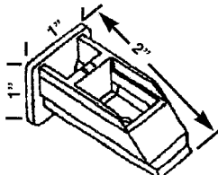
HWP 481 SASH CAM
