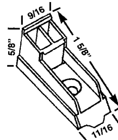
HWP 289 LOWER CAM
