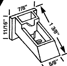
HWP 325 SASH CAM
