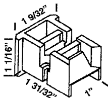
HWP 738 SASH GUIDE
