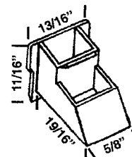
HWP 348 SASH CAM
