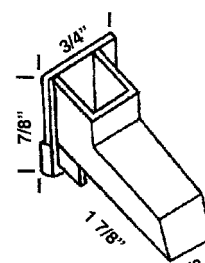
HWP 429 SASH CAM
