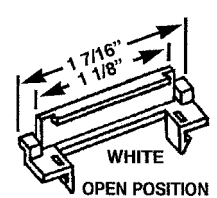
WHITE OPEN POSITION HWP 846 WEEP HOLE COVER
