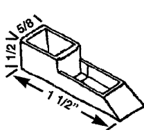
HWP 182 KINCO TOP GUIDE
