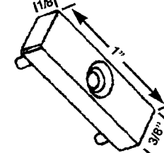
HWP 274 THERM GUIDE
