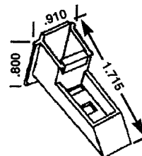
HWP 456 SASH CAM
