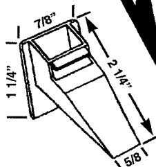
HWP 316 SASH CAM
