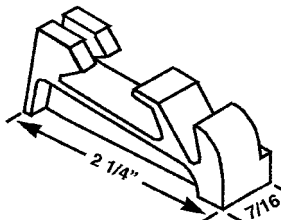
HWP 842 FRICTION SHOE SHOE
