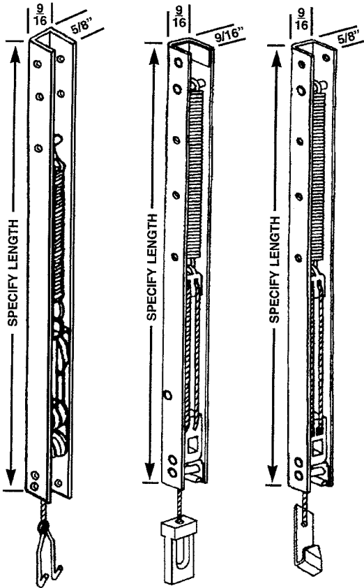
HWB-J 5/8" B & T BALANCE HWP 212 ATTACHED
