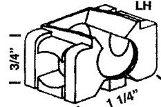
HWP 150 LEFT TERMINAL HOUSING
