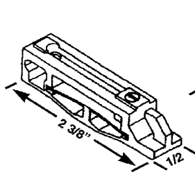
HWP 833 FRICTION SHOE
