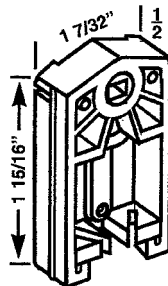
HWP 914 EFCO TILT HOUSING
