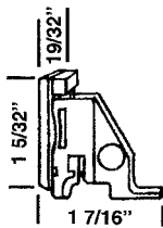
HWP 20 TUCKER SHOE
