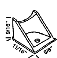
HWP 112 HARCAR TOP SASH GUIDE
