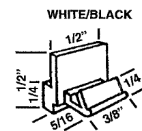
HWP 746 HARCAR 1901 SASH GUIDE WHITE/BLACK
