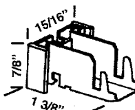
HWP 18 STANLEY SHOE
