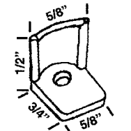
HWP 216 BALANCE GUIDE
