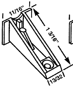
HWP 315 LOOK TOP GUIDE
