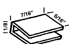
HWP 448 LIFT RAIL
