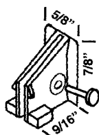
HWP 511 AIR CONTROL END SET W/FASTENERS
