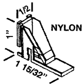
HWP 1 ABC/HARCAR FOOT
