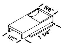
HWP 71 LATCH
