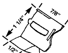
HWP 137 SUPERIOR SASH STOP
