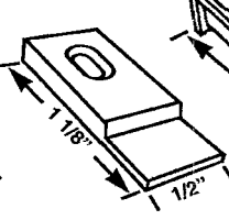
HWP 728
