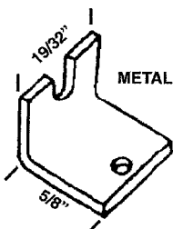
METAL HWP 881 ANGLE CLIP
