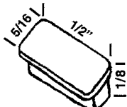
HWP 343 WARE
