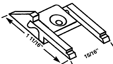
HWP 894 SPIRAL BALANCE GUIDE
