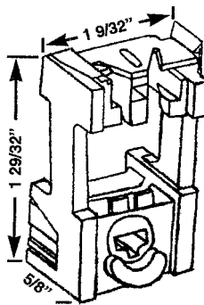
HWP 361 HOUSING
