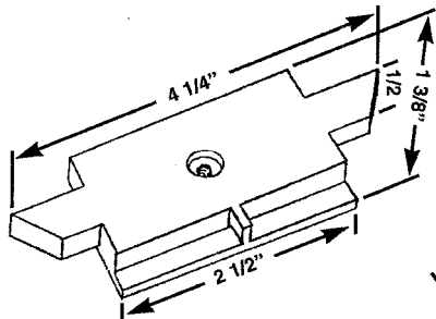
HWP 302 TILT LATCH
