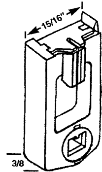
HWP 422 HOUSING
