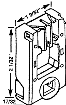
HWP 362 HOUSING
