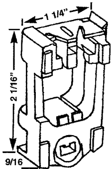
HWP 360 HOUSING
