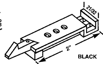
HWP 890 SLIDE LATCH
