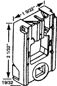
HWP 298 LOCK SHOE
