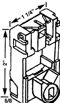
HWP 300 PIVOT SHOE
