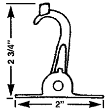
HWL 56 CROSSLY PULL
