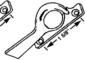
HWL 66 SWEEP LATCH
