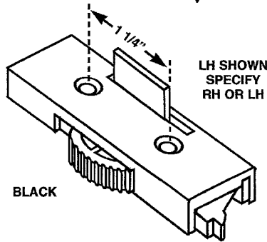
HWL 154 MILCO TILT LATCH
