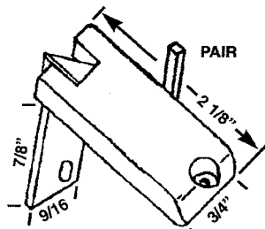
PAIR HWP 368 LATCH
