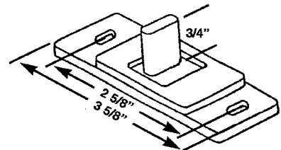
DSG 38 REAR RAIL BRACKET
