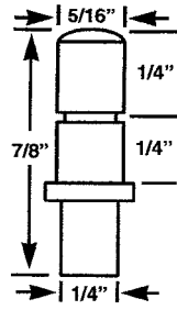
FAS 982 DOUBLE E-RING
