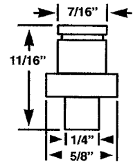
FAS 82 E-RING RIVET
