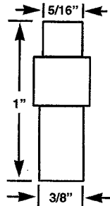
FAS 83 8-32 THREAD
