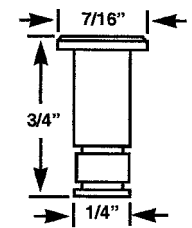
FAT 917 DOUBLE E-RING
