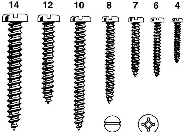
SLOTTED PHILLIPS
