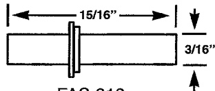
FAS 913 RIVET PIN W/SHOULDER
