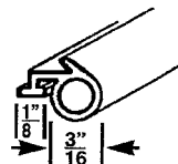
WDV 139 BULB VINYL ATW VENT
