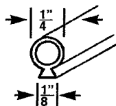
WDV 101 BULB VINYL .110 BASE
