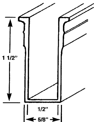
WDV 141 GLAZING CHANNEL
