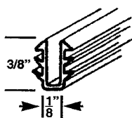
WDV 103 GLAZING BEAD
