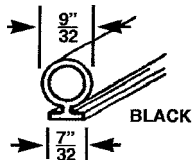
WDV 152 HEADER SILL VINYL
