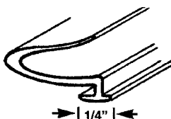
WDV 132 FLAP SEAL
