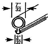
WDV 50 BULB VINYL
