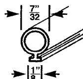
WDV 138 BULB VINYL
