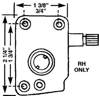
MHO 55 TORQUE LONG HUB
