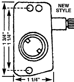
MHO 69 SIDEMOUNT
