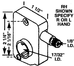
MHO 30 ROUND HUB
