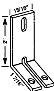
PDH 197 FIXED PANEL STOP W/SLOT
