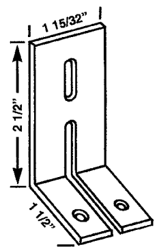
PDH 90 FIXED PANEL CLIP
