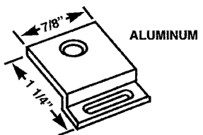
PDG 87 KELLER FIXED PANEL CLIP
