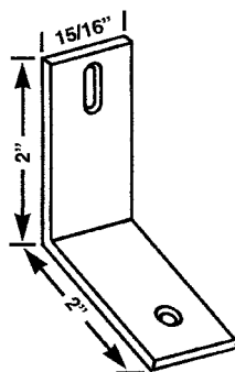
PDH 77 FIXED PANEL STOP
