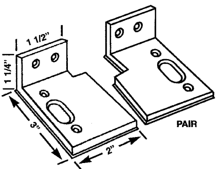
PDH 191 HOWARD FIXED PANEL STOP
