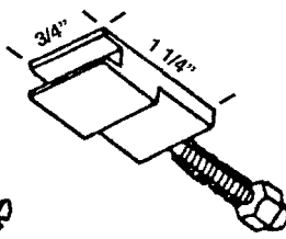
PDG 27 OLD PAN AM NARROW GUIDE
