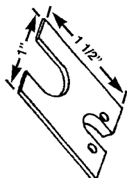
PDG 20 LAWSON/ CROWN GUIDE
