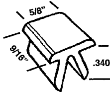
PDG 74 HEAD SPACER
