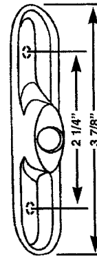
PDH 193 EXTERIOR PULL
