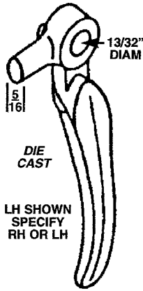
CWL 29 FENESTRA LOCKING HANDLE
