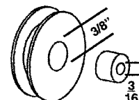
PSR 155 1 1/8" ROLLER & BUSHING
