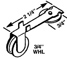
PSR 22 ARCADIA TOP RLR GUIDE
