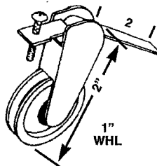
PSR 9 NYLON PSR 63 STEEL ADJ. RLR. ASMB
