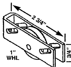
PSR 92 ALUMINUM BRACKET
