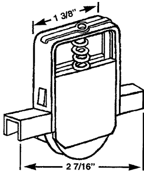
PSR 202 SCREEN ROLLER NYLON
