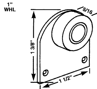
PSR 91 7/8" ROLLER & REPL. BRACKET
