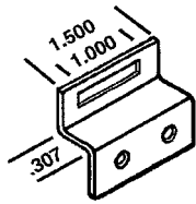
WSC 101 HANGER
