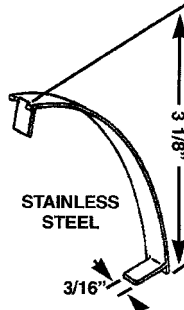
WSC 56 FLAT TENSION SPRING
