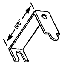
WSC 150 5/8" "C" CLIP
