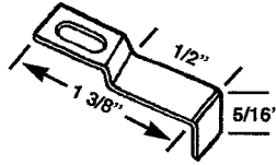
WSC 2 MODIFIED "L" CLIP
