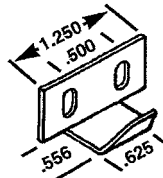
WSC 100 HANGER
