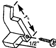
WSC 93 ACORN LATCH
