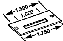
WSC 156 STRIKE
