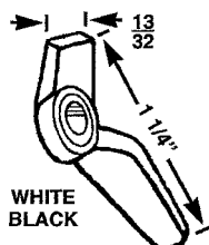
WSC 70 SWIVEL LATCH
