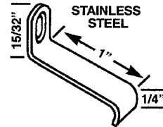
WSC 180 "Z" CLIP
