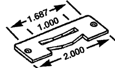
WSC 97 STRIKE
