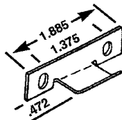
WSC 102 HANGER
