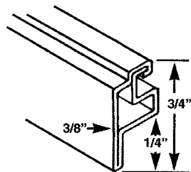
WSS 55 3/8" x 3/4" 19 GAUGE 12'6" STOCK LGTHS. 170 PCS./2125' PER CTN.
