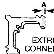
EXTRUDED CORNER LOCK A WCK 68 .192" WCK 69 .313"
