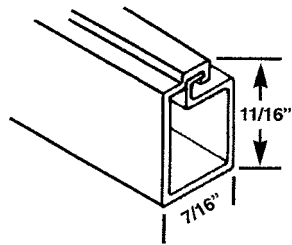
WSS 15 7/16" x 1 1/16" 19 GAUGE 12'6" STOCK LGTHS. 120 PCS./1500' PER CTN.
