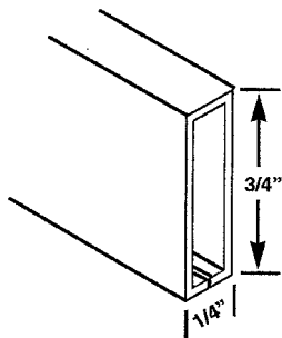
WSS 20 CROSS BRACE 1/4" x 3/4" 19 GAUGE 12'6" STOCK LGTHS.
