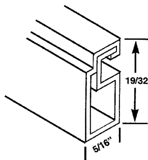
WSS 12 5/16" x 19/32" 19 GAUGE 12'6" STOCK LGTHS.
